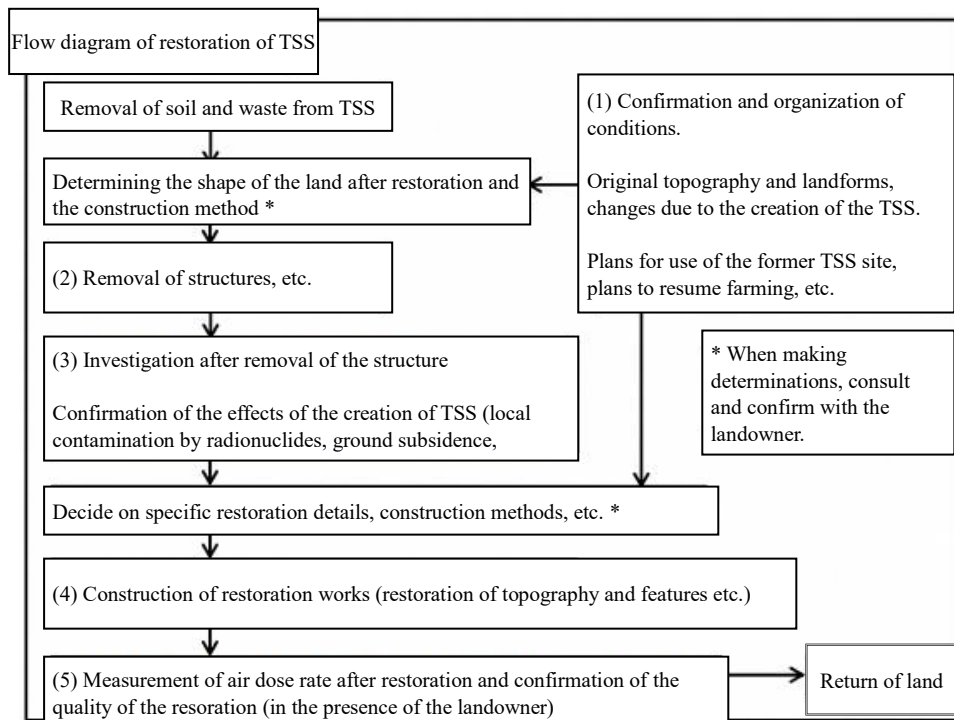
Figure 6. Flow diagram of restoration of TSS 2
