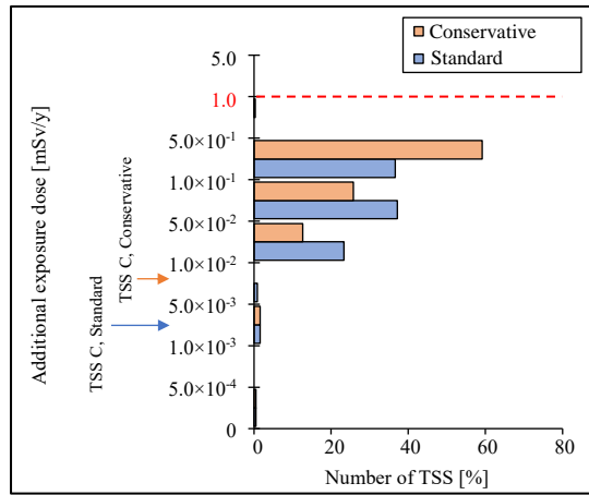
Figure 17. Additional exposure dose using estimated 137 Cs (Residence scenario (Adult))
