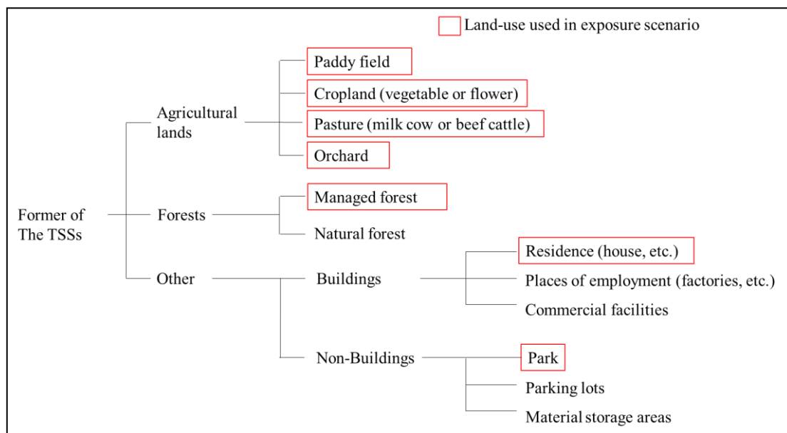
Figure 7: The land-use assumed for the former TSS
