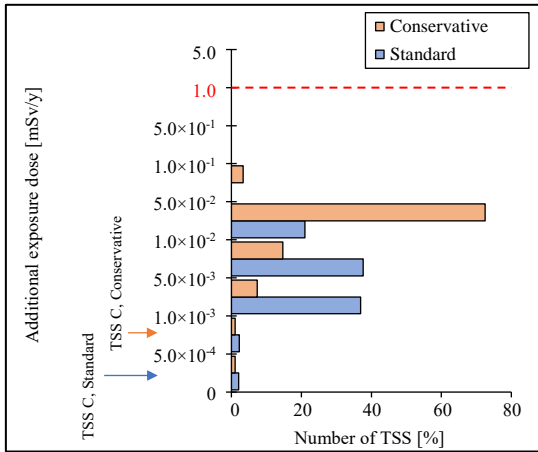
Figure 18. Additional exposure dose using estimated 137 Cs (Park scenario (Adult))
