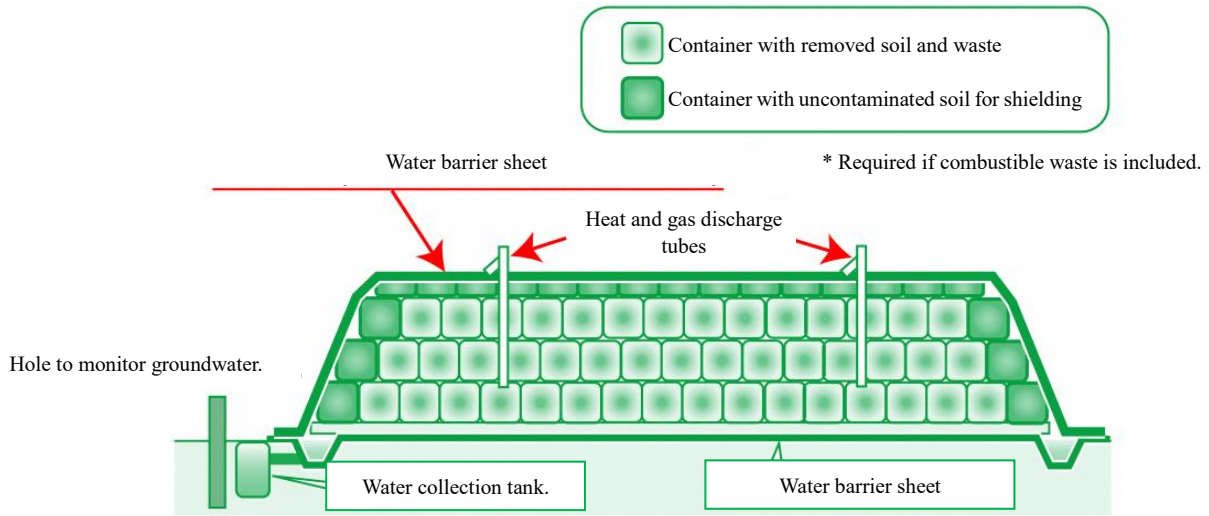
Figure 3. Basic design and structure of TSS 8
