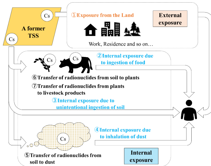
Figure 8. Illustration of potential exposure pathways
