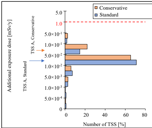
Figure 12. Additional exposure dose using estimated ^{137}\text{Cs} (Cropland (flower) scenario (Adult))
