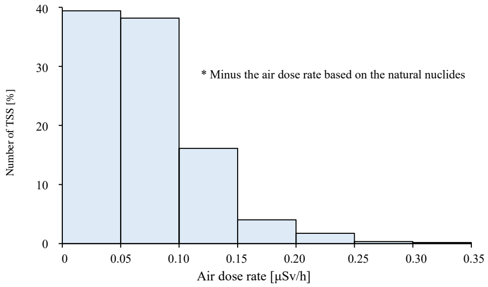
Figure 9. The probability distribution of the measured air dose rates at the TSS
