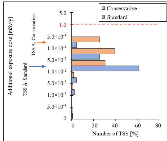
Figure 11. Additional exposure dose using estimated ^{137}\text{Cs} (Cropland (vegetable) scenario (Adult))
