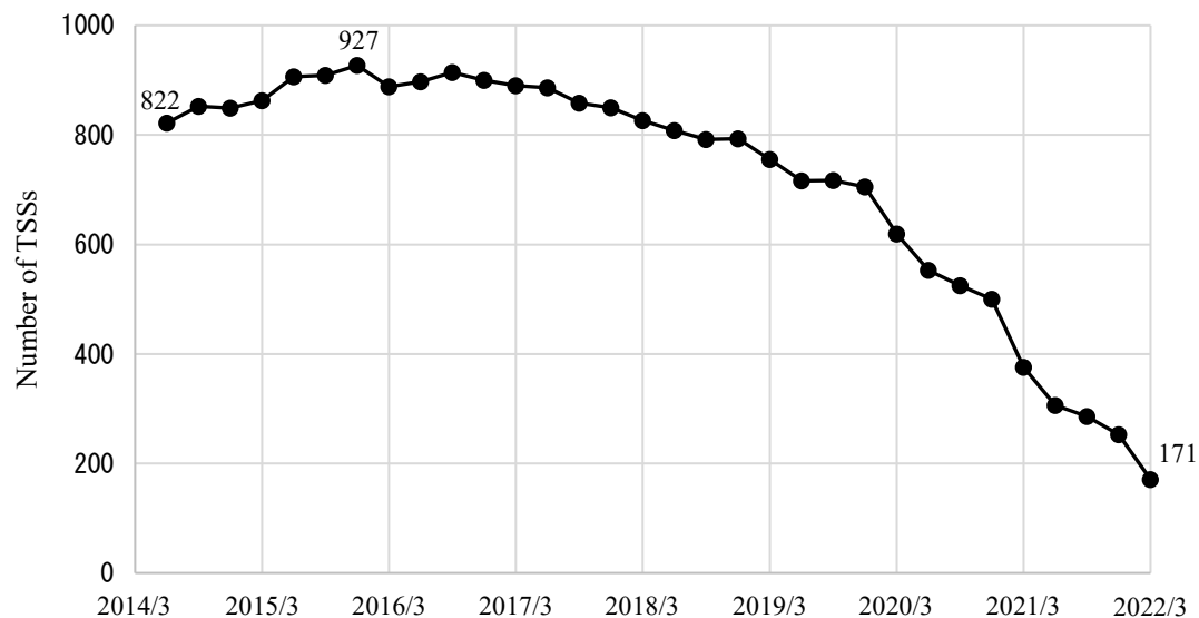
Figure 5. Number of TSSs of ICSA in Fukushima Prefecture over time 9
