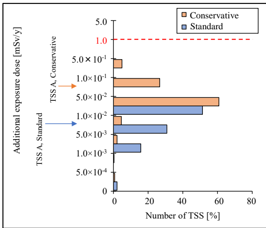
Figure 10. Additional exposure dose using estimated ^{137}\text{Cs} (Paddy scenario (Adult))
