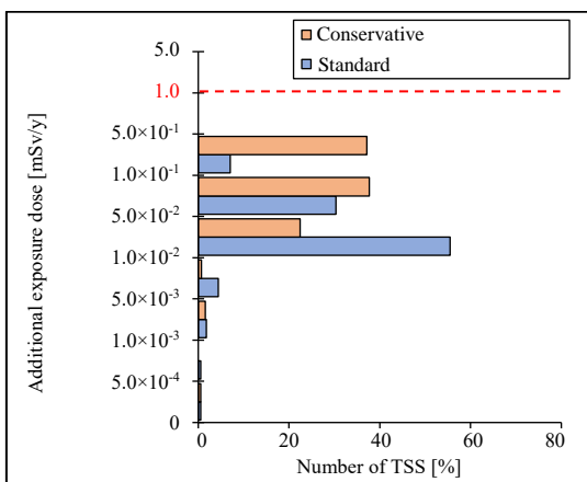
Figure 14. Additional exposure dose using estimated ^{137}\text{Cs} (Pasture (milk cow) scenario (Adult))
