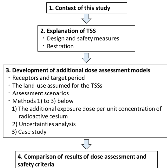
Figure 2. Flow diagram of dose assessment in the present study
