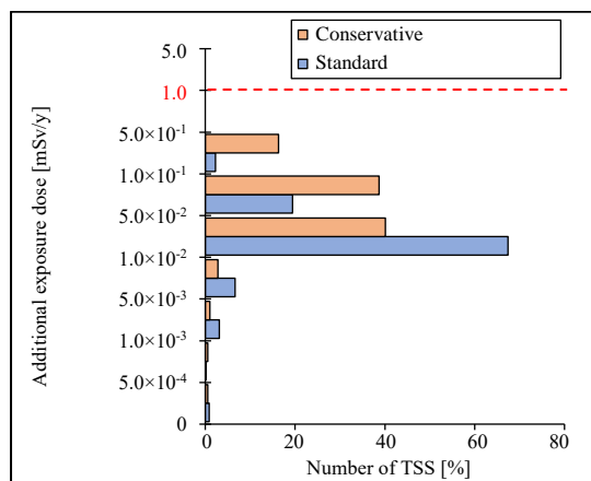
Figure 15. Additional exposure dose using estimated ^{137}\text{Cs} (Pasture (beef cattle) scenario (Adult))
